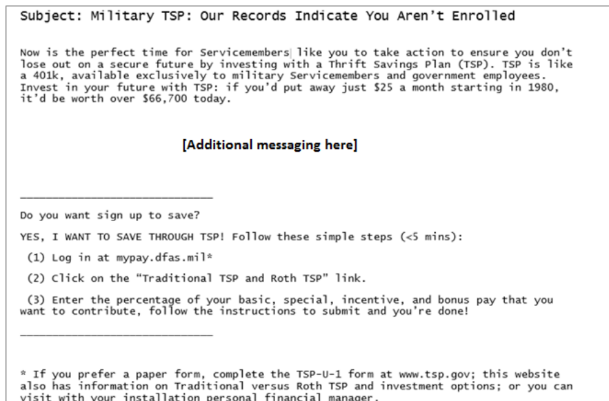
Figure 1: Sample Message
